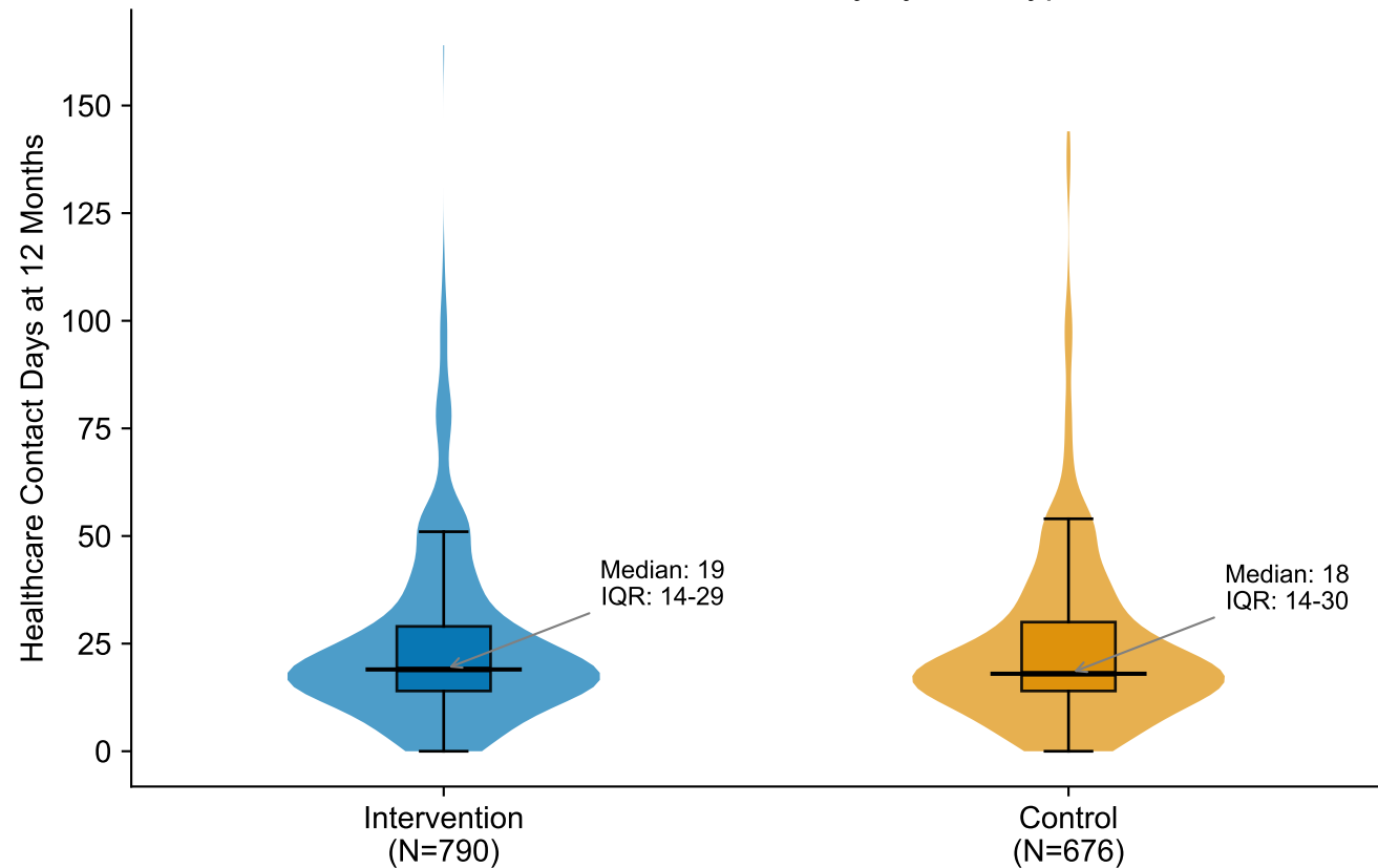
Distribution of Time Toxicity by Arm Type
